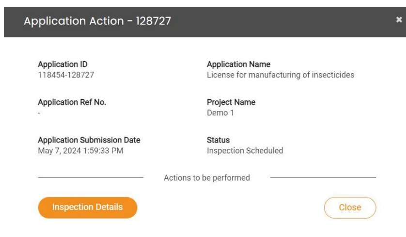
Figure 29. 'Inspection Scheduled'
