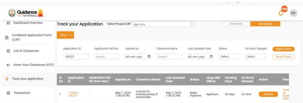
Figure 19. Make Payment
