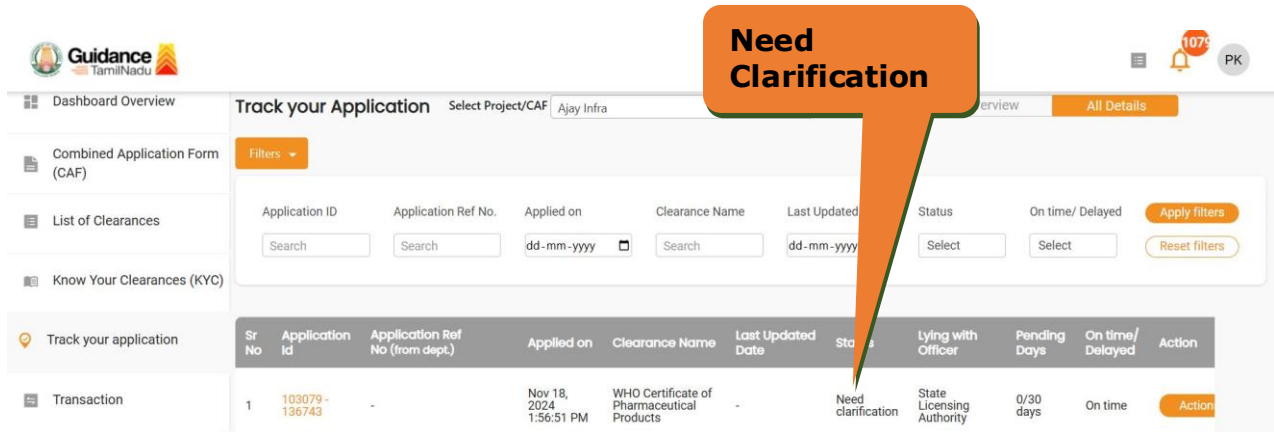
Figure 26. Need Clarification
