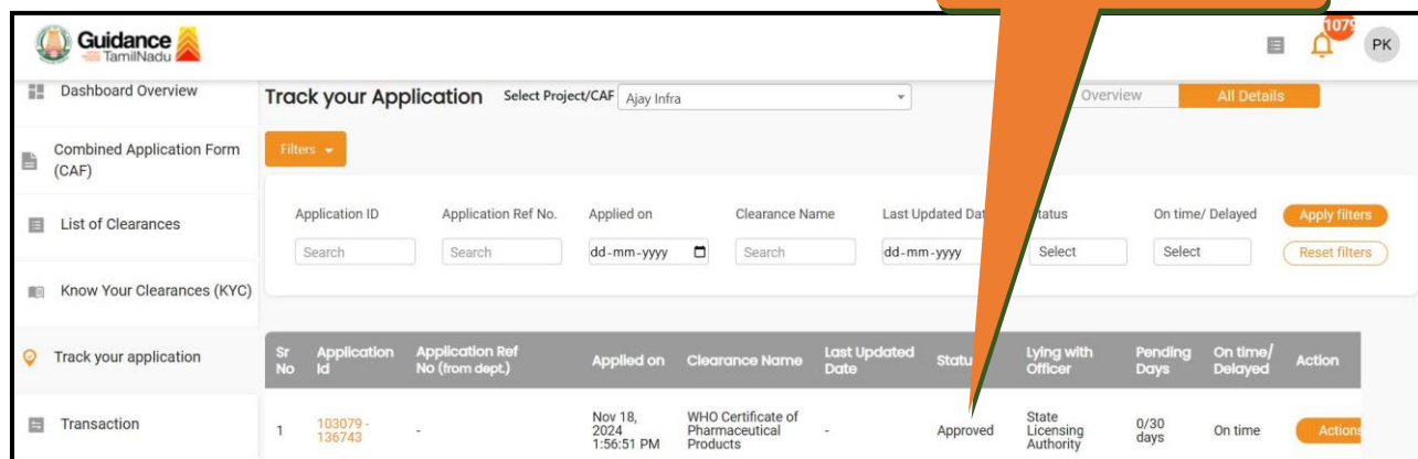
Figure 31. Application Processed
