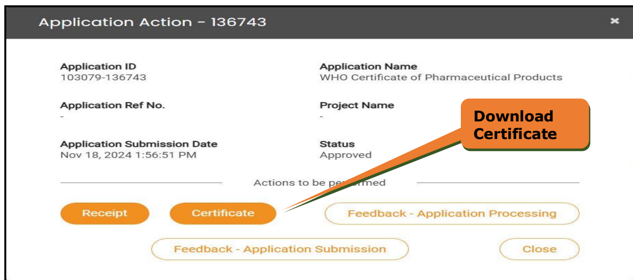
Figure 32. Download Certificate
