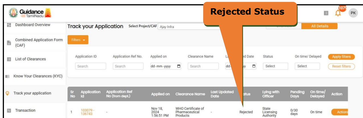
Figure 33. Rejected Status
