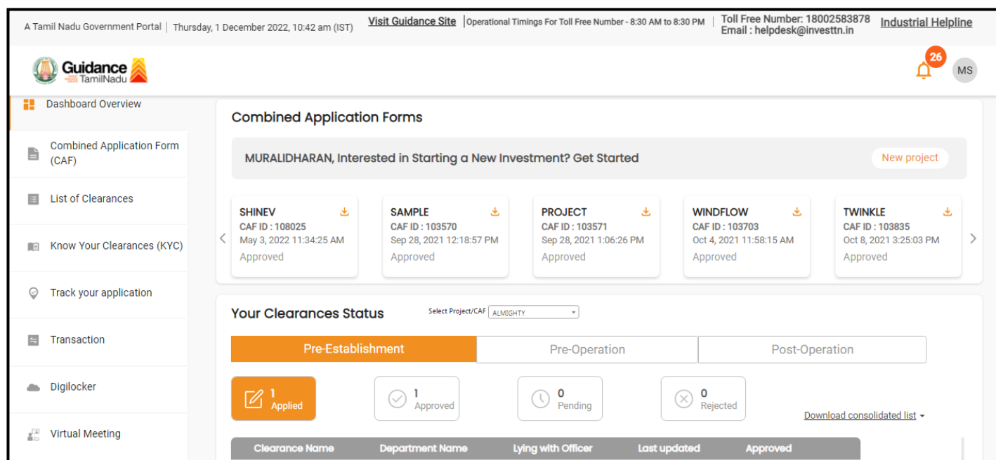
Figure 9. Dashboard Overview
