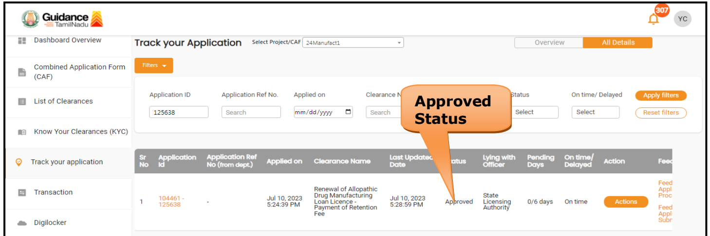
Figure 25. Application Processed
