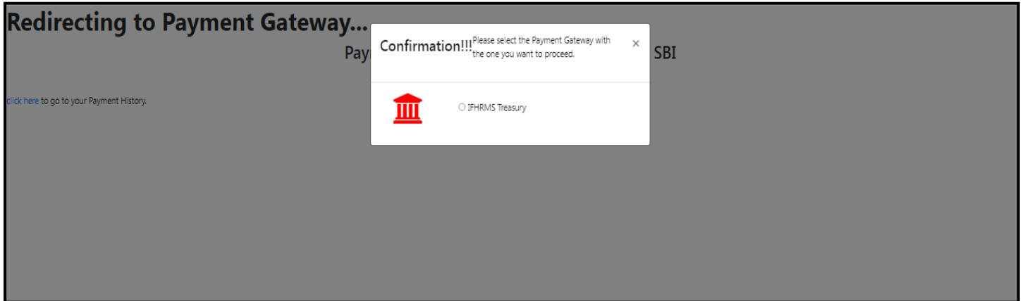
Figure 20. Payment Process
